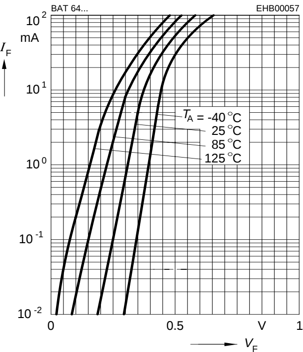
Forward current I_F = f(V_F) T_A = \text{Parameter}
