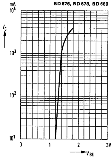
Collector current I_C = f(V_{BE}) -V_{CE} = 3 \text{ V}; T_{case} = 25^\circ\text{C}
