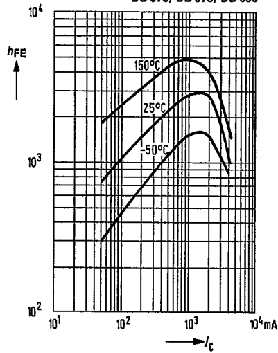
DC current gain h_{FE} = f(I_C) -V_{CE} = 3 \text{ V}
