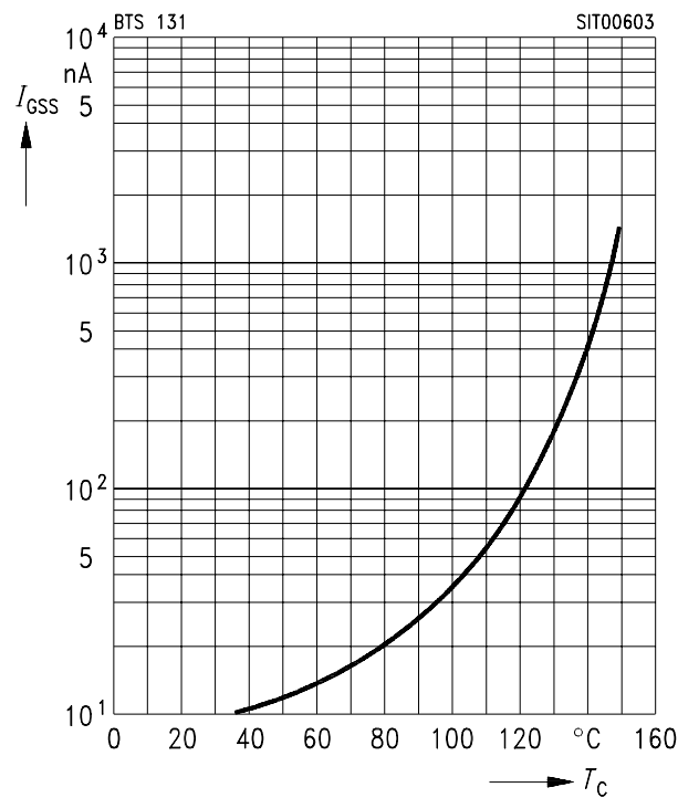
Typ. gate-source leakage current I_{GSS} = f(T_C) Parameter: V_{GS} = 10 \text{ V}, V_{DS} = 0
