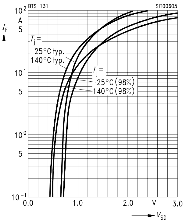
Forward characteristics of reverse diode I_F = f(V_{SD}) Parameter: T_j, t_p = 80 \mu\text{s} (spread)
