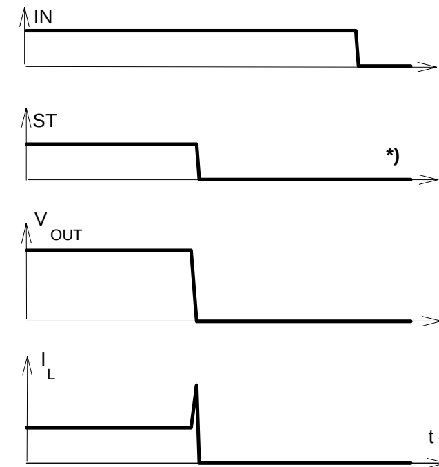
Figure 4a: Overtemperature: Reset if T_j < T_{jt}
