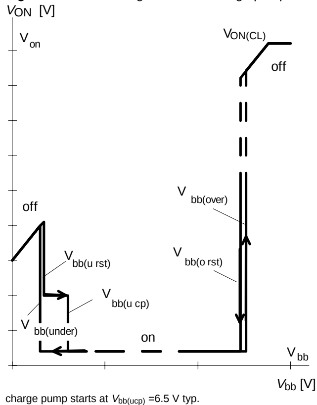
Figure 7a: Overvoltage:
