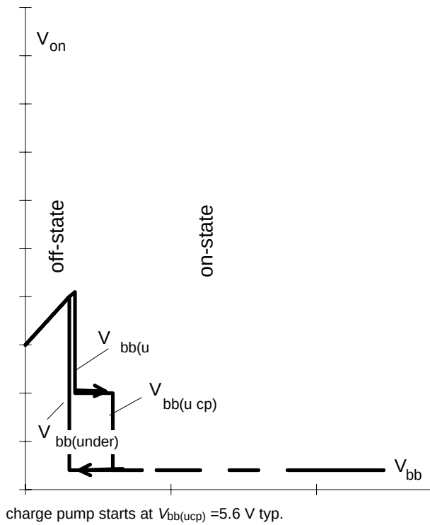
Figure 7a: Overvoltage, no shutdown:
