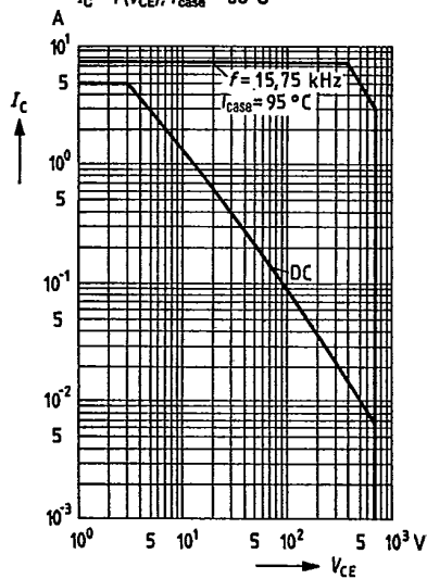
Permissible operating range I_C = f(V_{CE}) ; T_{case} = 95^\circ\text{C}
