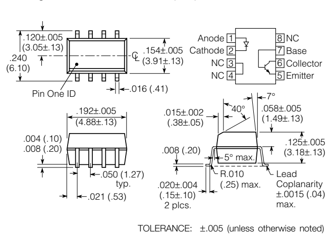
Package Dimensions in Inches (mm)
