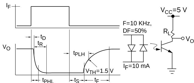
Figure 14. Switching timing and schematic
