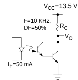
Figure 9. Switching schematic
