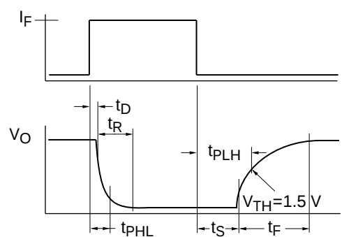
Figure 10. Switching waveform
