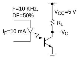
Figure 3. Saturated switching timing
