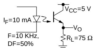
Figure 1. Non-saturated switching timing
