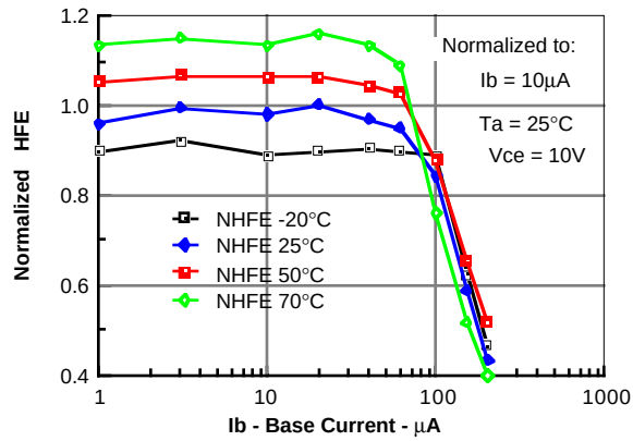
Figure 9. Normalized HFE versus Ib, Ta
