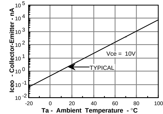
Figure 12. Collector-emitter leakage current versus temperature
