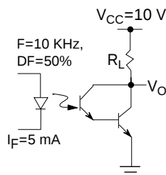
Figure 7. Switching schematic
