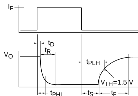
Figure 6. Switching timing
