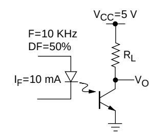
Figure 10. Non-saturated switching schematic
