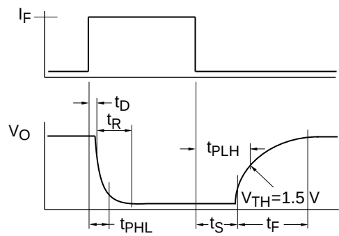
Figure 9. Switching timing
