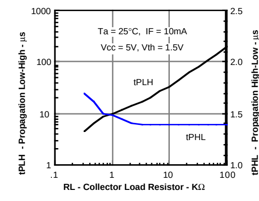
Figure 19. -4 Propagation delay versus collector load resistor
