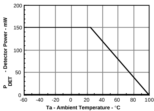
Figure 14. Maximum detector power dissipation
