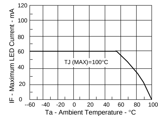
Figure 5. Maximum LED current versus ambient temperature
