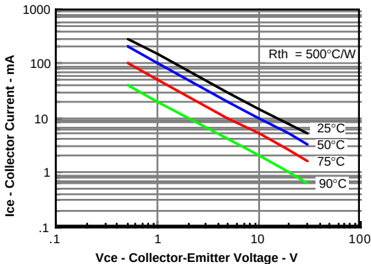
Figure 12. Maximum collector current versus collector voltage
