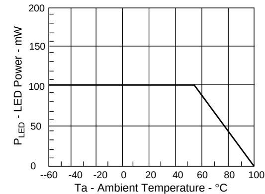
Figure 6. Maximum LED power dissipation
