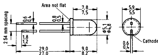
Package Dimensions mm
