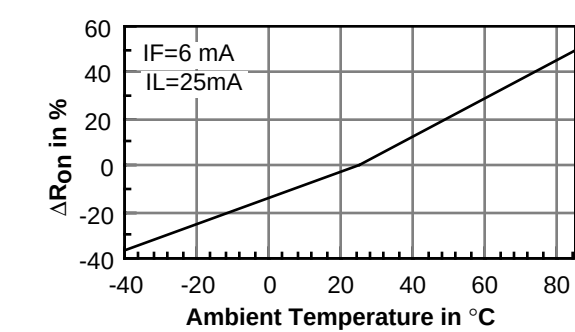
Figure 9. \Delta R_{on} vs. temperature
