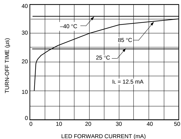
C. Turn-Off Time vs. LED Current (LH1544)
