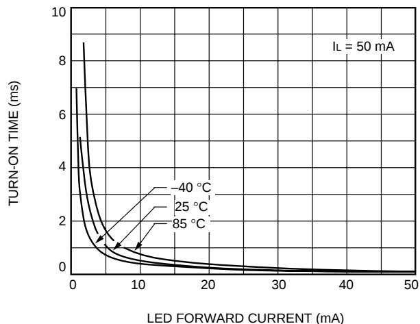
D. Turn-On Time vs. LED Current
