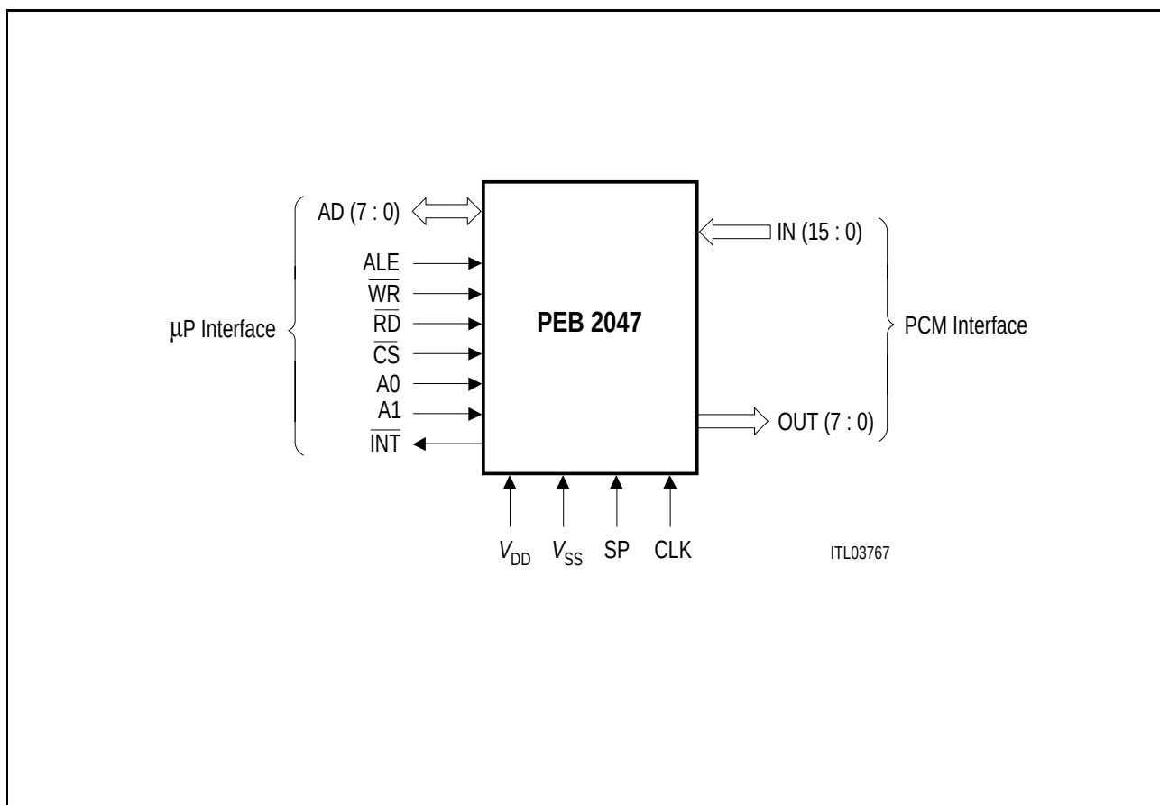
Figure 1 Functional Symbol
