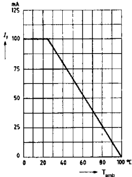
Maximum permissible forward current I_F = f(T_{amb})
