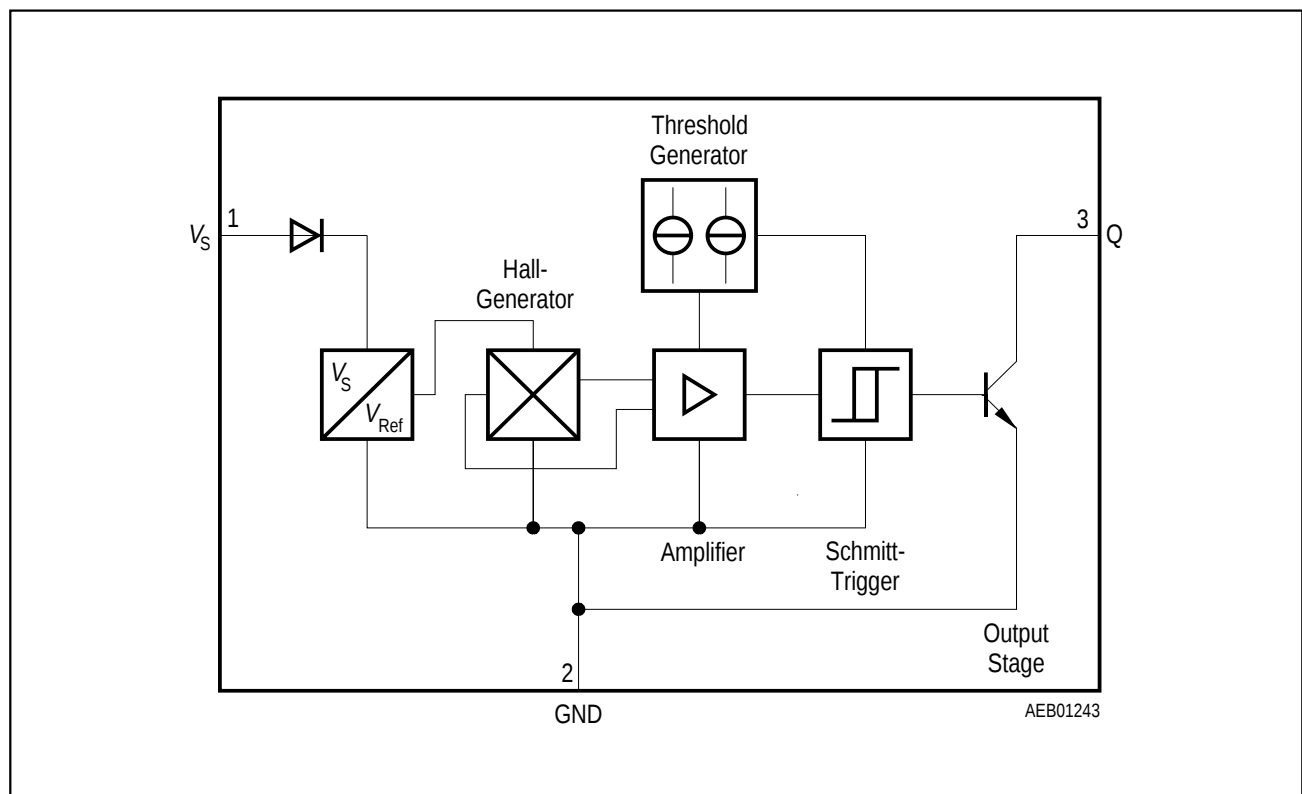
Figure 2 Block Diagram
