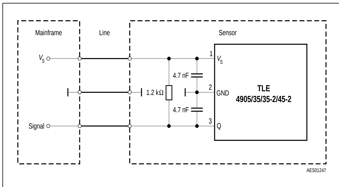
Figure 8 Application Circuit
