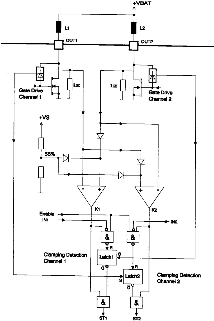
Block Diagram of Open Load Detection
