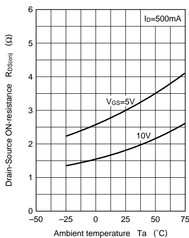
R_{DS(on)} - T_a
