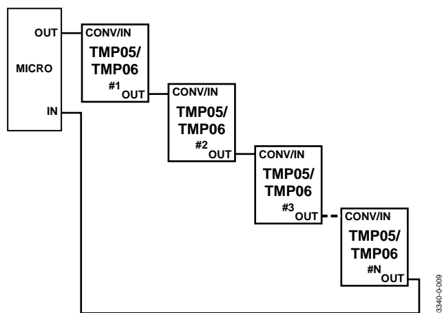
Figure 25. Daisy-Chain Structure
