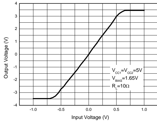
Figure 8. Spindle Driver Characteristics
