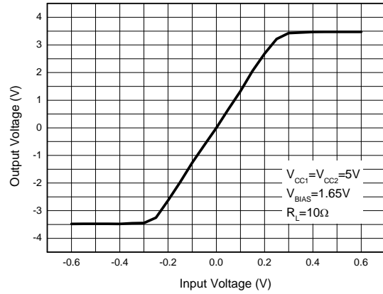
Figure 6. Tracking Driver Characteristics
