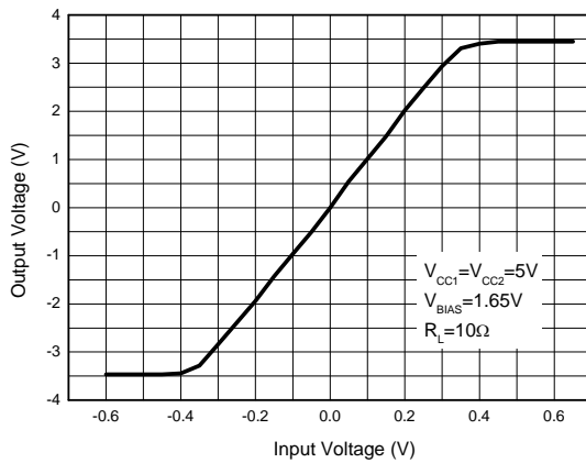
Figure 7. Sled Driver Characteristics
