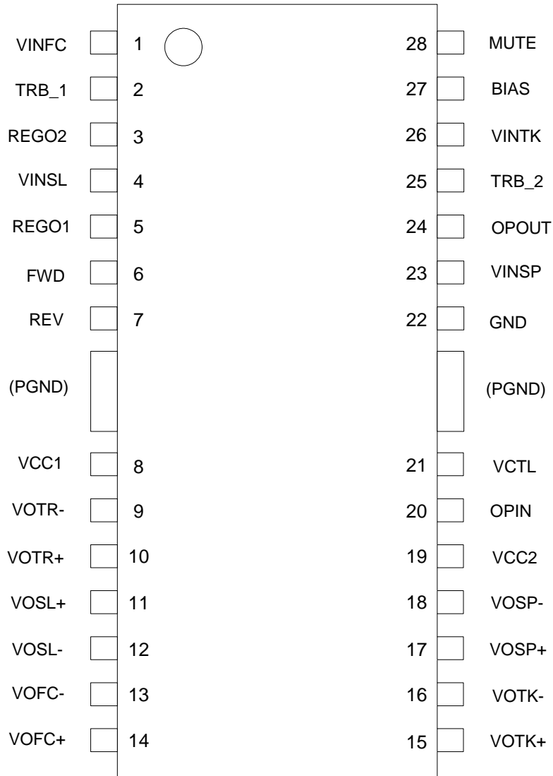
Figure 2. Pin Configuration of AM5669 (Top View)
