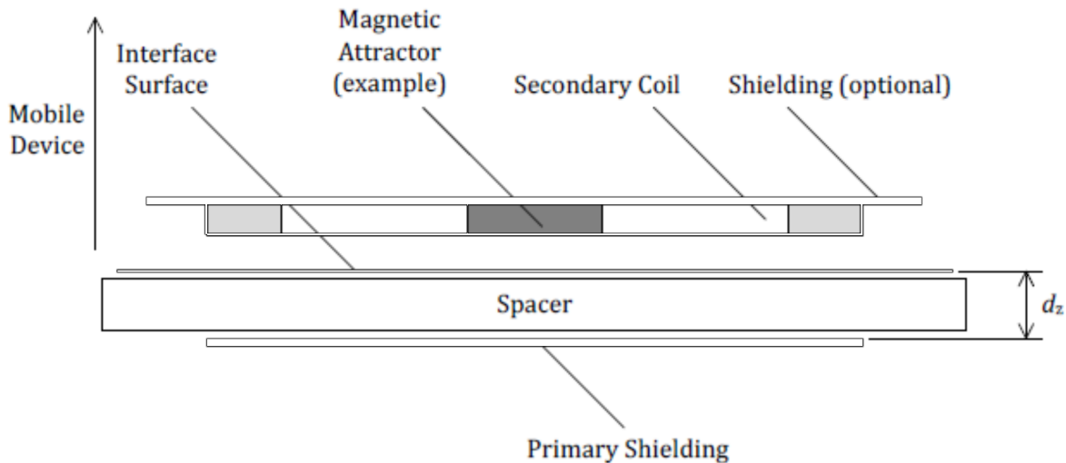
Figure 31. WPC v1.0 Receiver Coil Test Fixture for the Inductance Measurement L_{s'} (copied from System Description Wireless Power Transfer, volume 1: Low Power, Part 1 Interface Definition, Version 1.0.1, Figure 4-4)
