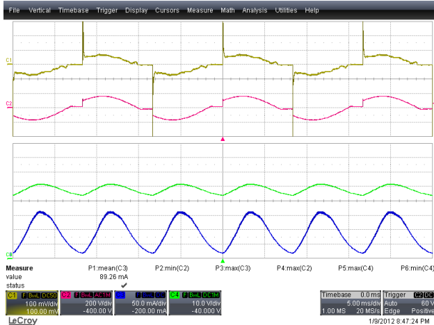
Figure 66 – Full Conduction. Ch1: I_{IN} , 100 mA / div. Ch2: V_{IN} , 200 V / div. Ch3: I_{OUT} , 50 mA / div. Ch4: V_{OUT} , 10 V / div. Time Scale: 5 ms / div.
