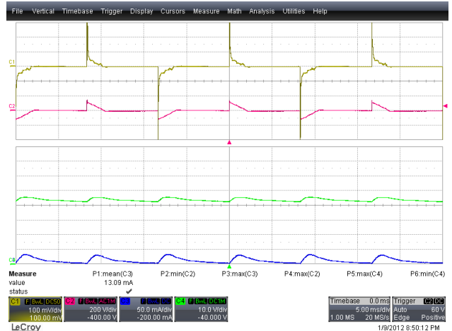
Figure 69 – 45 Degrees. Ch1: I_{IN} , 100 mA / div. Ch2: V_{IN} , 200 V / div. Ch3: I_{OUT} , 50 mA / div. Ch4: V_{OUT} , 10 V / div. Time Scale: 5 ms / div.
