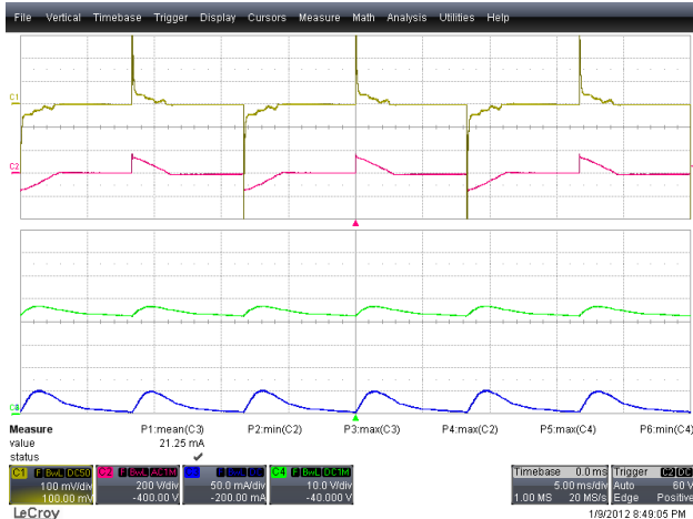
Figure 68 – 60 Degrees. Ch1: I_{IN} , 100 mA / div. Ch2: V_{IN} , 200 V / div. Ch3: I_{OUT} , 50 mA / div. Ch4: V_{OUT} , 10 V / div. Time Scale: 5 ms / div.
