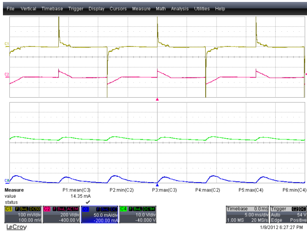
Figure 65 – 45 Degrees. Ch1: I IN , 100 mA / div. Ch2: V IN , 200 V / div. Ch3: I OUT , 50 mA / div. Ch4: V OUT , 10 V / div. Time Scale: 5 ms / div.
