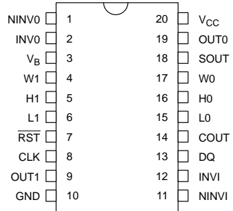
20-Pin DIP (300 Mil) and 20-Pin SOIC
