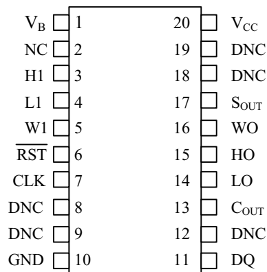
20-Pin TSSOP (173-mil) See Mech. Drawings Section
