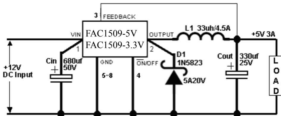
Figure 11. Typical Application of FAC1509 For 3.3V 5V
