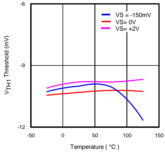
Fig 6. V_{TH1} vs. Temp. and Common Mode (OVT=Floating)
