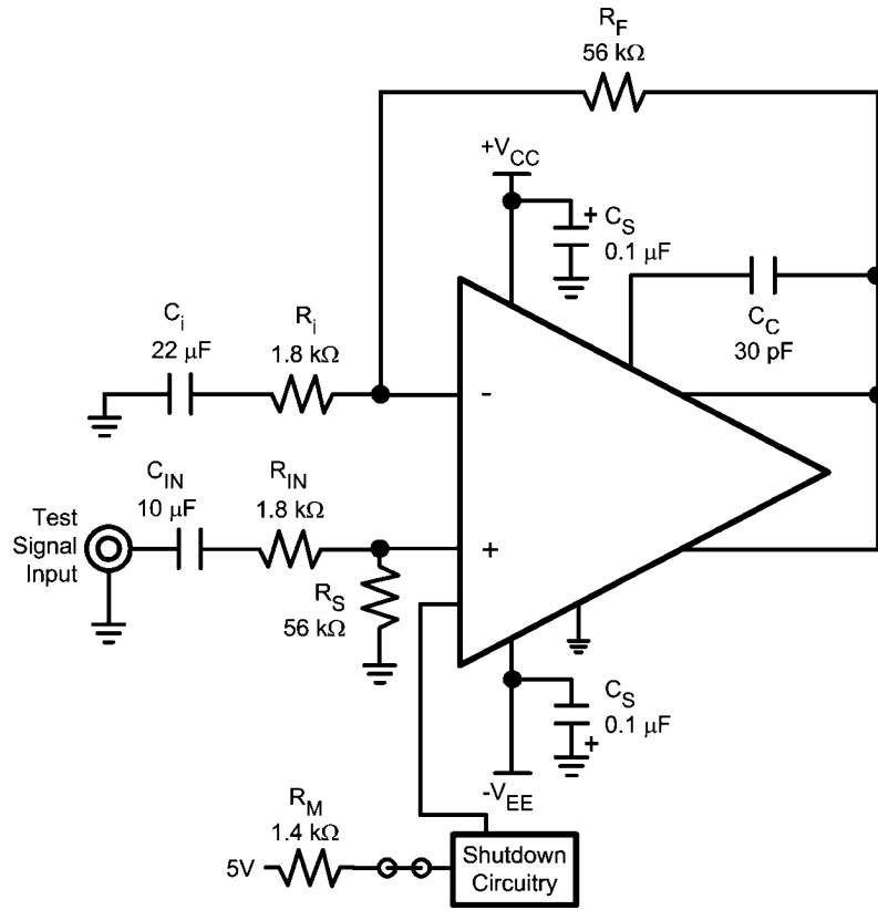
FIGURE 3. Test Circuit
