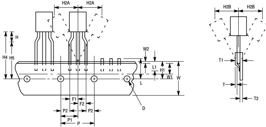
Figure 12. Device Positioning on Tape
