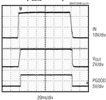
STARTUP AND DISABLE FROM IN ( R_{LOAD} = 3.3k\Omega )
