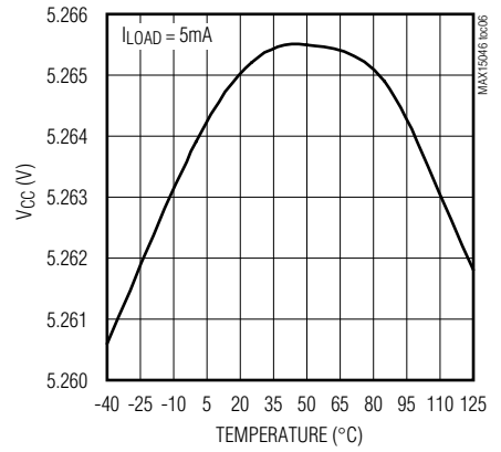
VCC vs. TEMPERATURE
