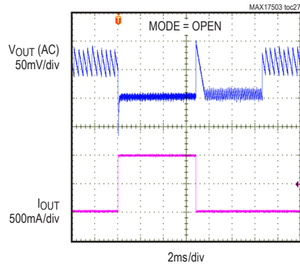
3.3V OUTPUT, DCM MODE (LOAD CURRENT STEPPED FROM 50mA TO 1A), FIGURE 4 CIRCUIT
