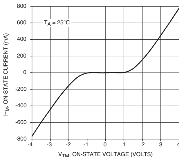
Figure 6. On-State Characteristics
