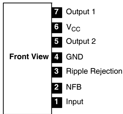
Pin Connection Diagram
