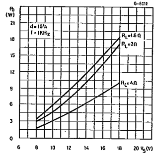
Fig. 6 - Output power vs. supply voltage
