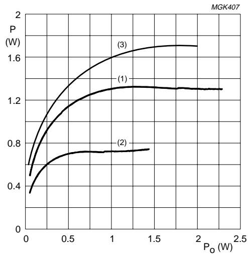
Sine wave of 1 kHz. (1) V_{CC} = 9\text{ V} , R_L = 16\ \Omega . (2) V_{CC} = 5\text{ V} , R_L = 8\ \Omega . (3) V_{CC} = 7.5\text{ V} , R_L = 8\ \Omega .
