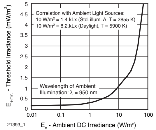
Fig. 6 - Sensitivity in Bright Ambient
