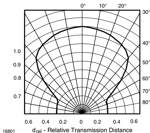
Fig. 12 - Directivity
