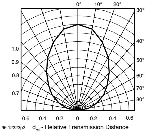
Fig. 10 - Directivity
