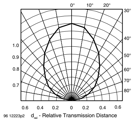
Figure 12. Directivity
