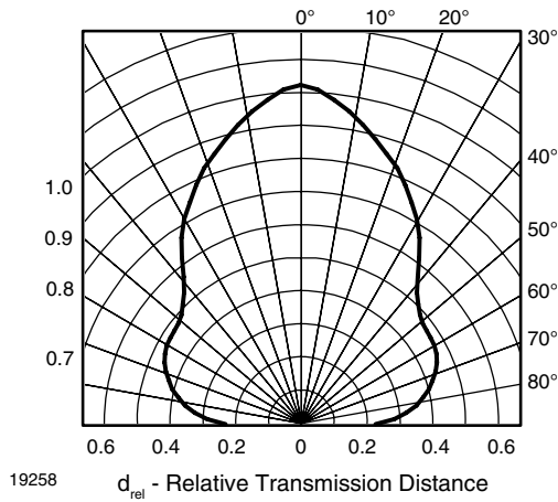
Fig. 10 - Horizontal Directivity
