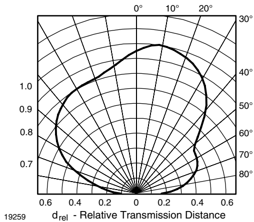
Fig. 11 - Vertical Directivity
