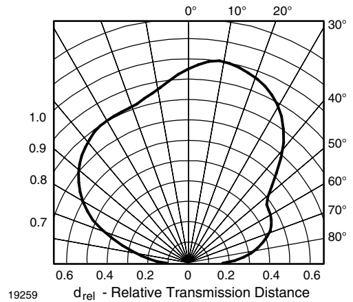
Fig. 13 - Vertical Directivity
