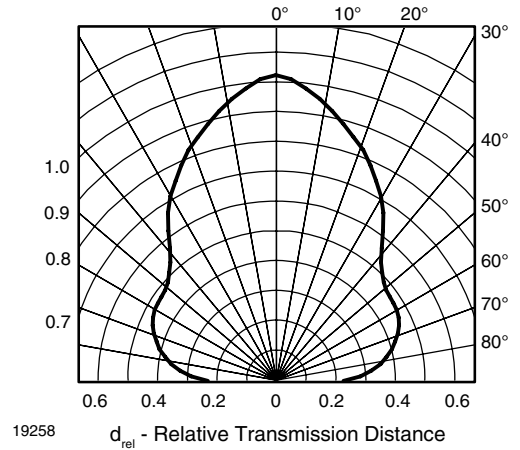
Fig. 12 - Horizontal Directivity
