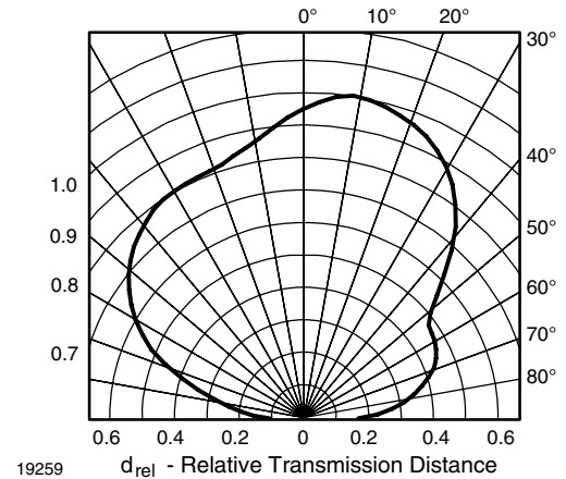
Fig. 13 - Vertical Directivity
