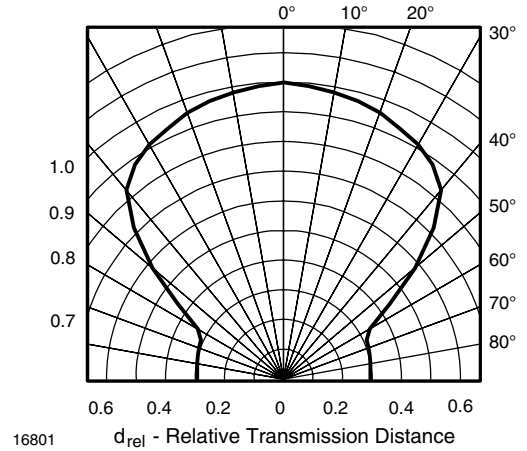
Fig. 12 - Directivity
